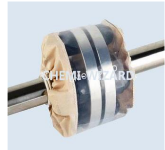
BH2 泄漏保护套 BH2 Safety Shield
